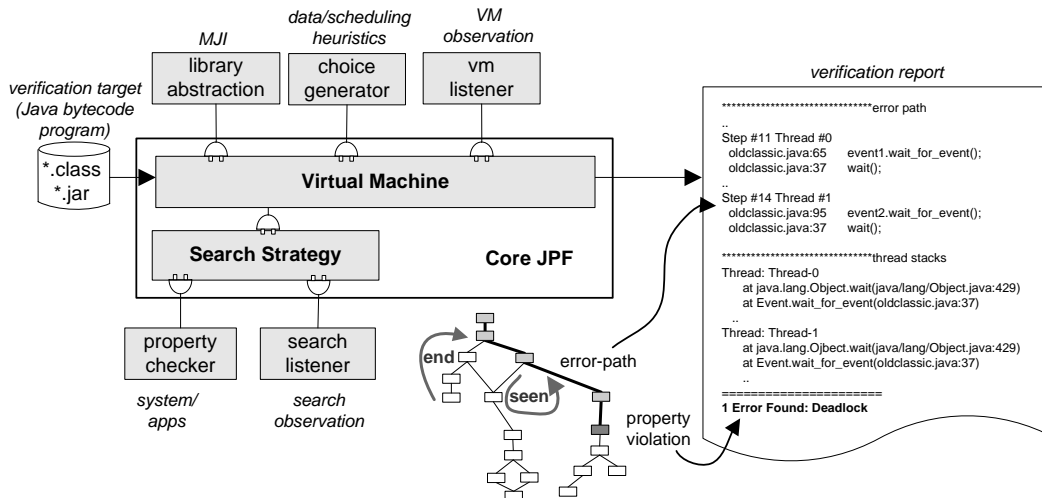
Figure 3. Model Checking with Java PathFinder [1]
