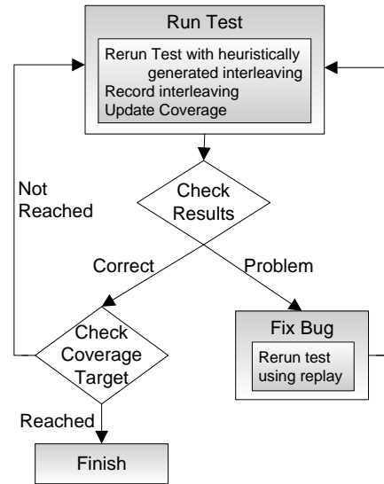
Figure 2. Testing with ConTest [11]
